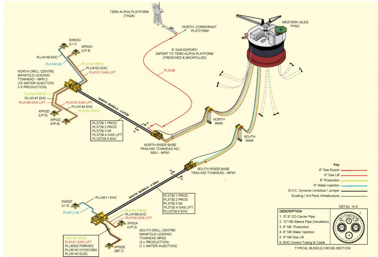
Figure 2-1 Western Isles (Barra and Harris) fields layout
