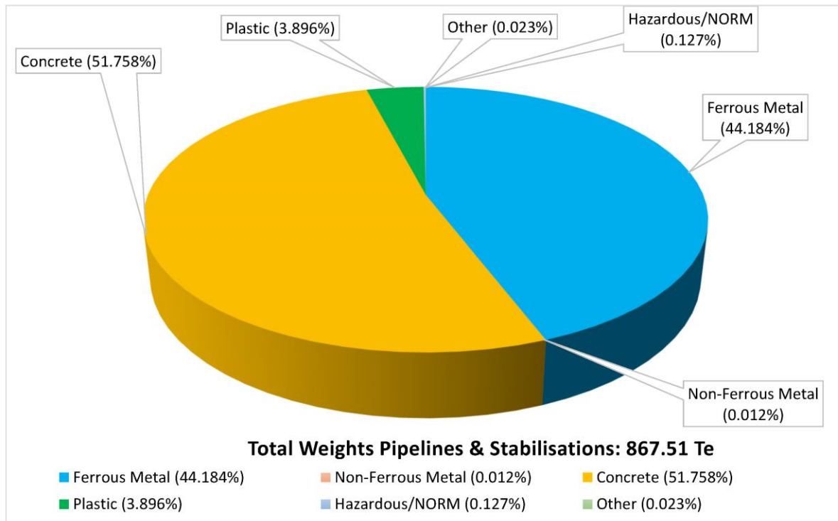
Figure 3-7 Pie chart of the estimated material inventory for the subsea pipeline and stabilisations
