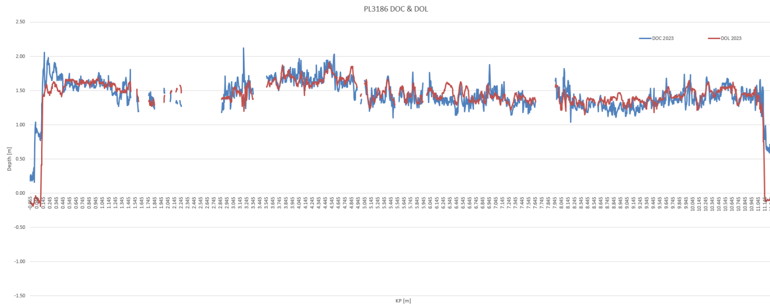
Figure E.3 PL3186 Depth of burial (2023) 7
