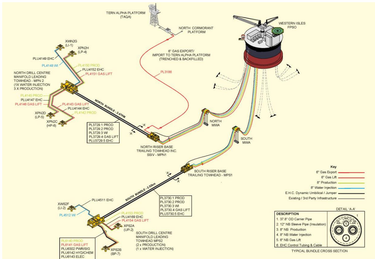
Figure 1-2 Western Isles facilities layout 1
