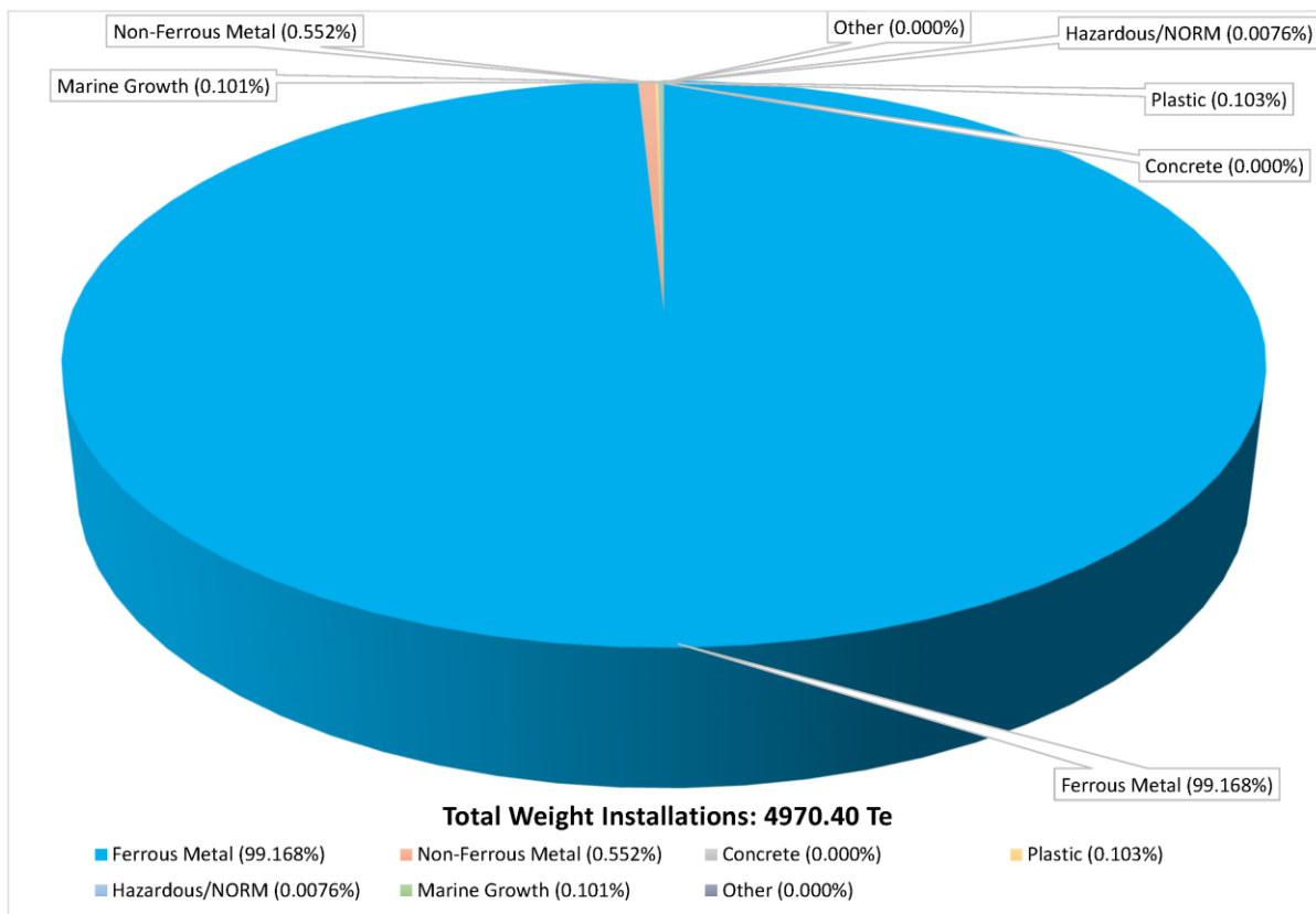
Figure 3-6 Pie chart of estimated material inventory for the subsea installations
